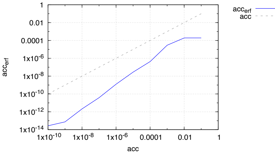
accuracy of erf(1) for different acc
